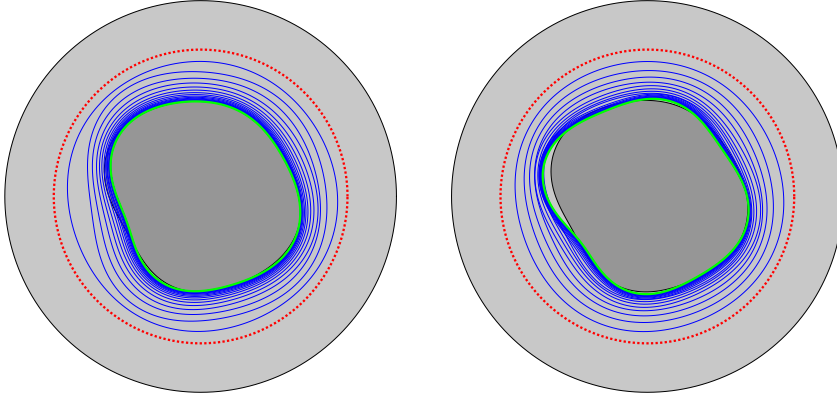
FIG. 3. Iterates (in thin blue lines) and the final reconstructions for the second example (in green thick line) with 1% noise (left-hand side) and with 5% noise (right-hand side).
