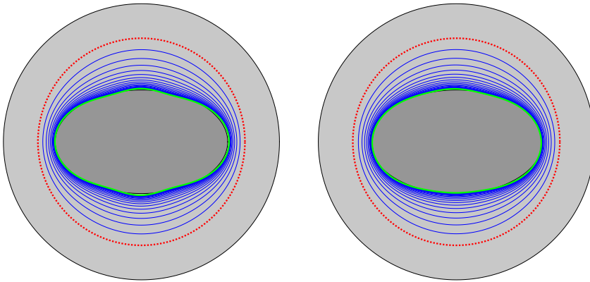
FIG. 2. Iterates (in thin blue lines) and the final reconstructions (in green thick line) for different scalings of a kite shaped void with 1% noise.
