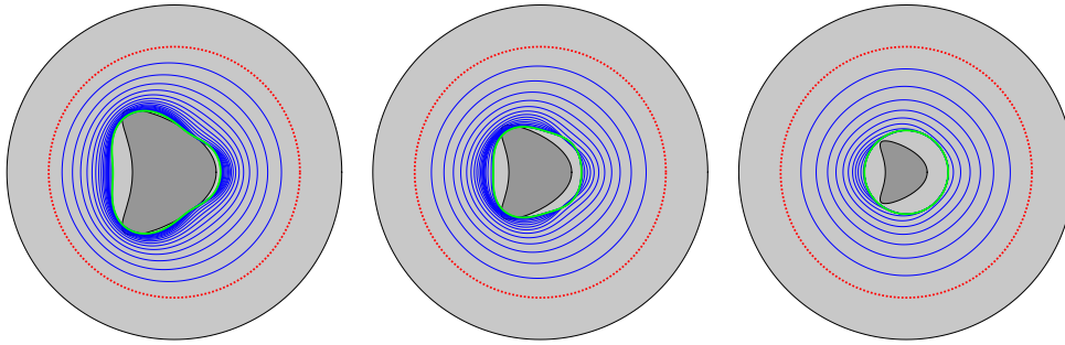
FIG. 5. Iterates (in thin blue lines) and the final reconstructions for the non-convex case (in green thick line) with 1% noise (left-hand side) and with 5% noise (right-hand side).
